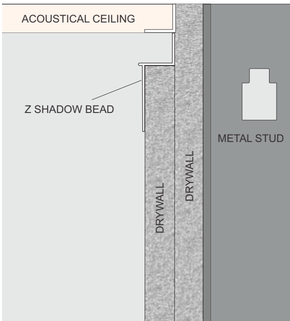
Ceiling Detail
